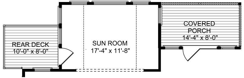
SUNROOM w/ DECK & COVERED PORCH OPTION
